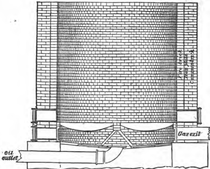
Coke Oven.—Section.
